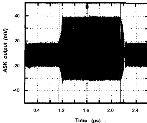
Fig. 4. Time domain ASK output of the hybrid version of BPSK to ASK Converter in response to two consecutive phase changes of the BPSK signal.
